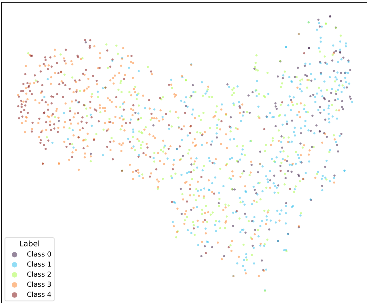
google/bert_uncased_L-2_H-128_A-2-sst5-SOFT4-TRIPa2-3 (val)
