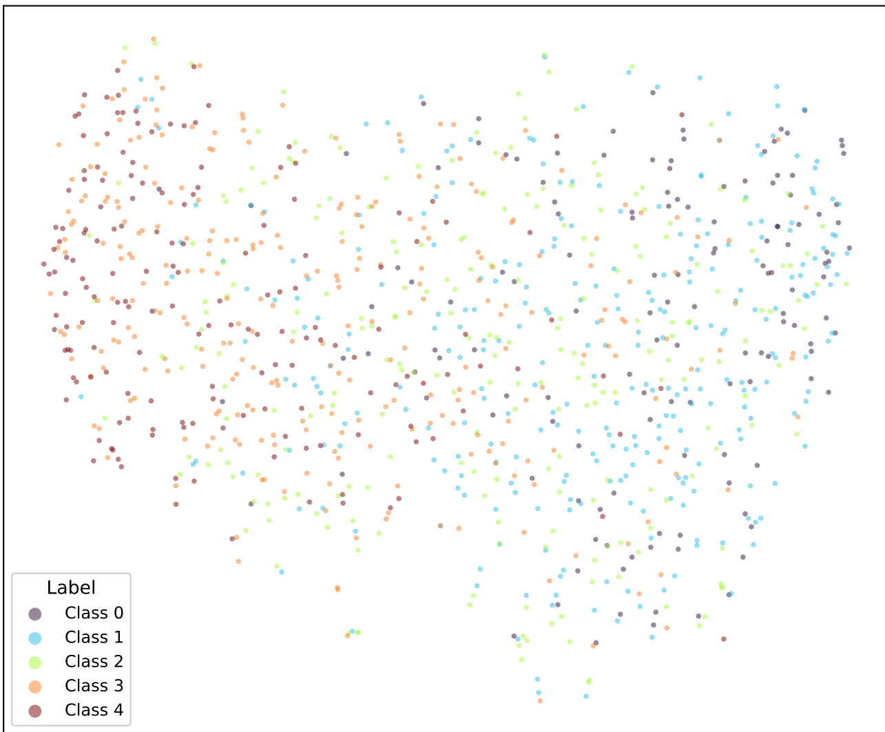
google/bert_uncased_L-2_H-128_A-2-sst5-SOFT4-TRIPa2-4 (val)
