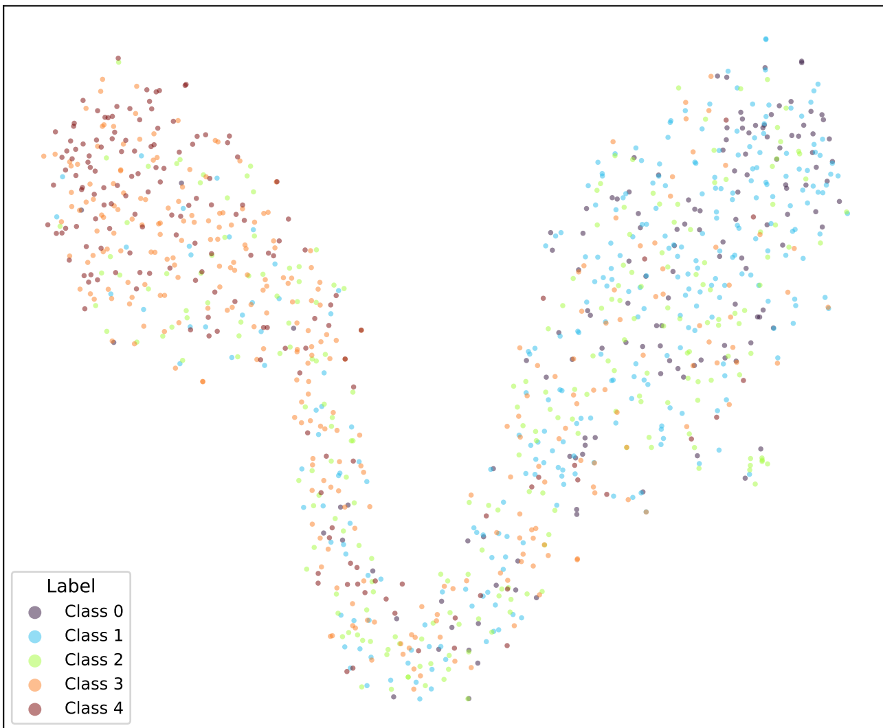
google/bert_uncased_L-2_H-128_A-2-sst5-WKL-TRIPa1-1 (val)
