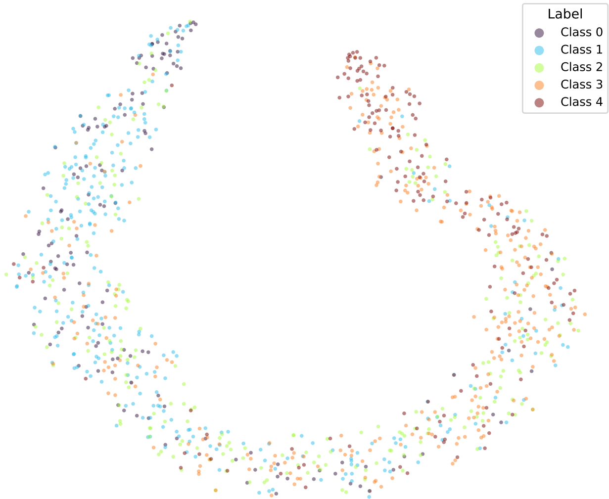
google/bert_uncased_L-2_H-128_A-2-sst5-WKL-TRIPa1-3 (val)
