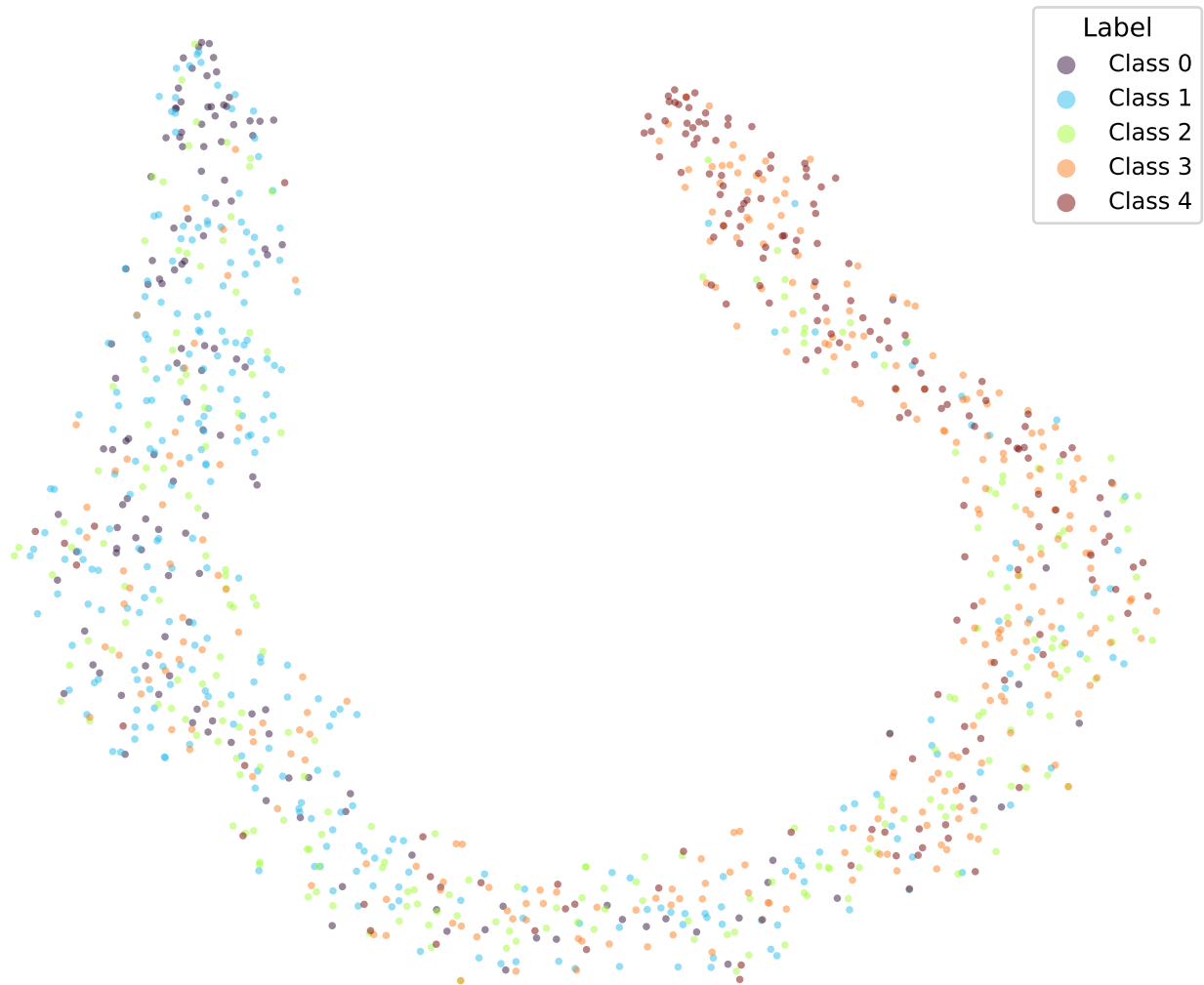
google/bert_uncased_L-2_H-128_A-2-sst5-WKL-TRIPa2-3 (val)
