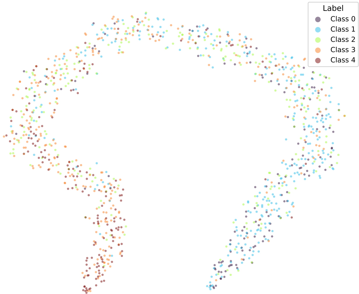
google/bert_uncased_L-2_H-128_A-2-sst5-WKL-TRIPa2-5 (val)
