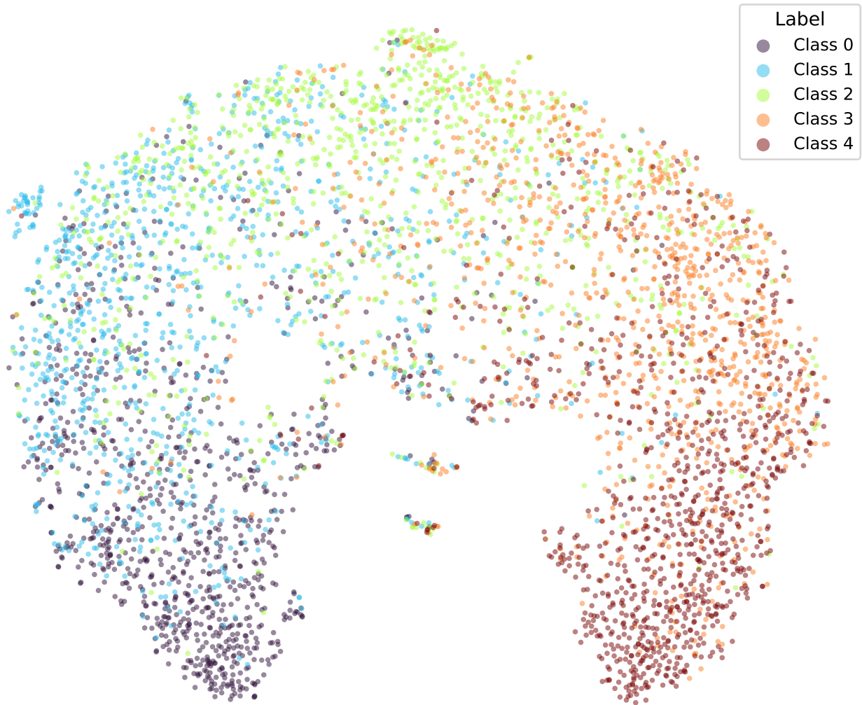
google/bert_uncased_L-2_H-128_A-2-yelp-BCE-TRIPa1-2 (val)
