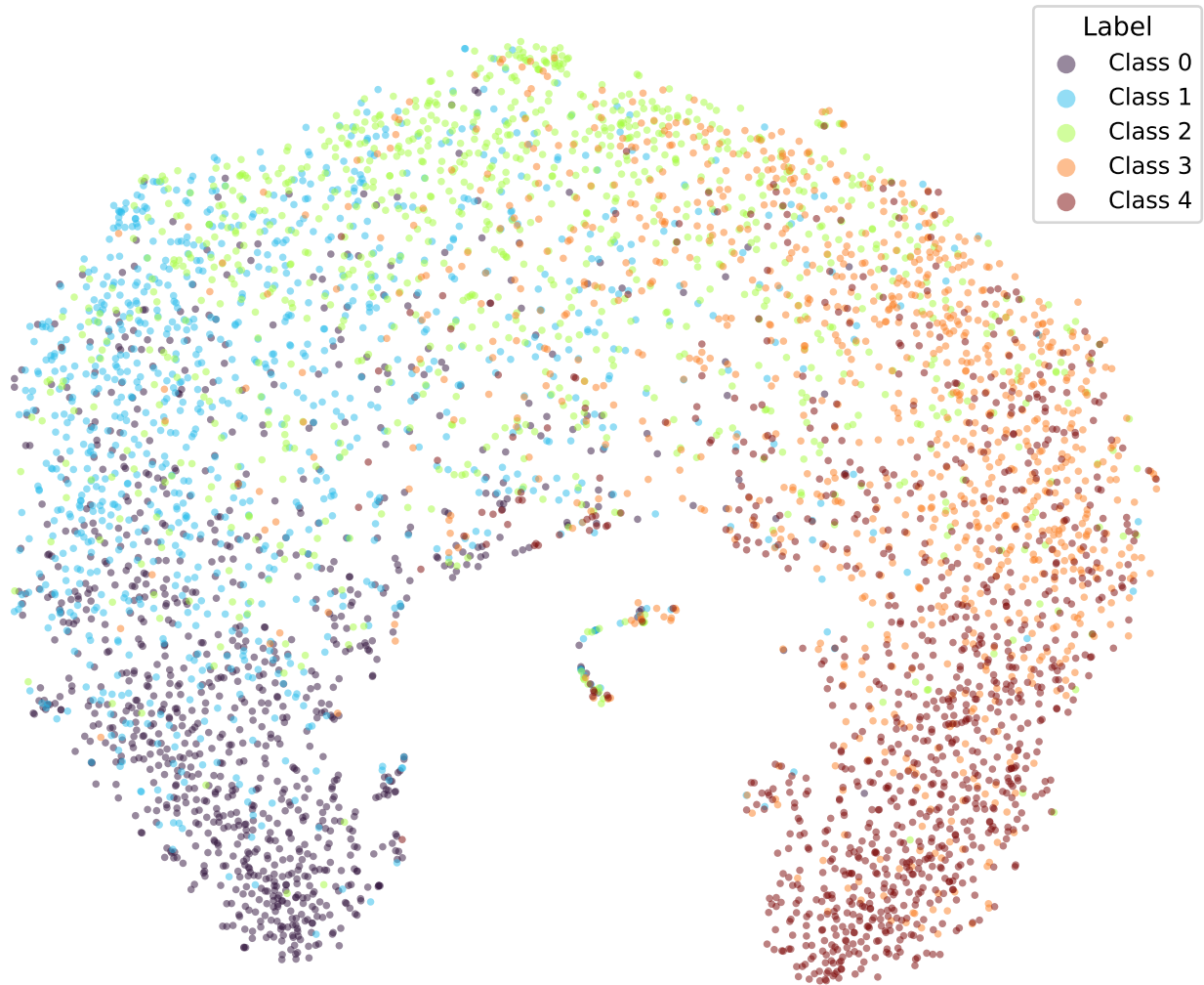
google/bert_uncased_L-2_H-128_A-2-yelp-BCE-TRIPa2-1 (val)
