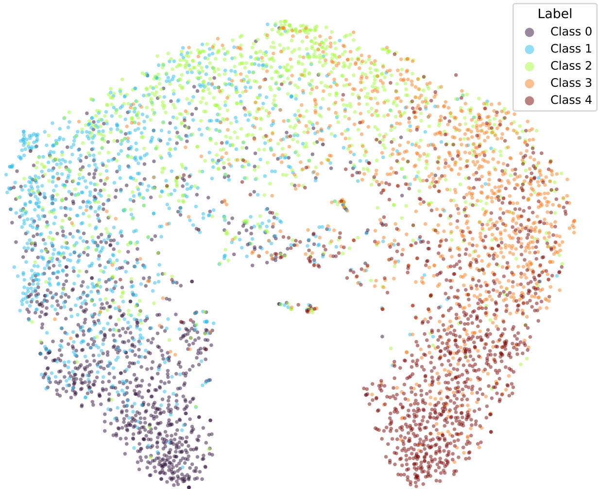
google/bert_uncased_L-2_H-128_A-2-yelp-BCE-TRIPa2-2 (val)
