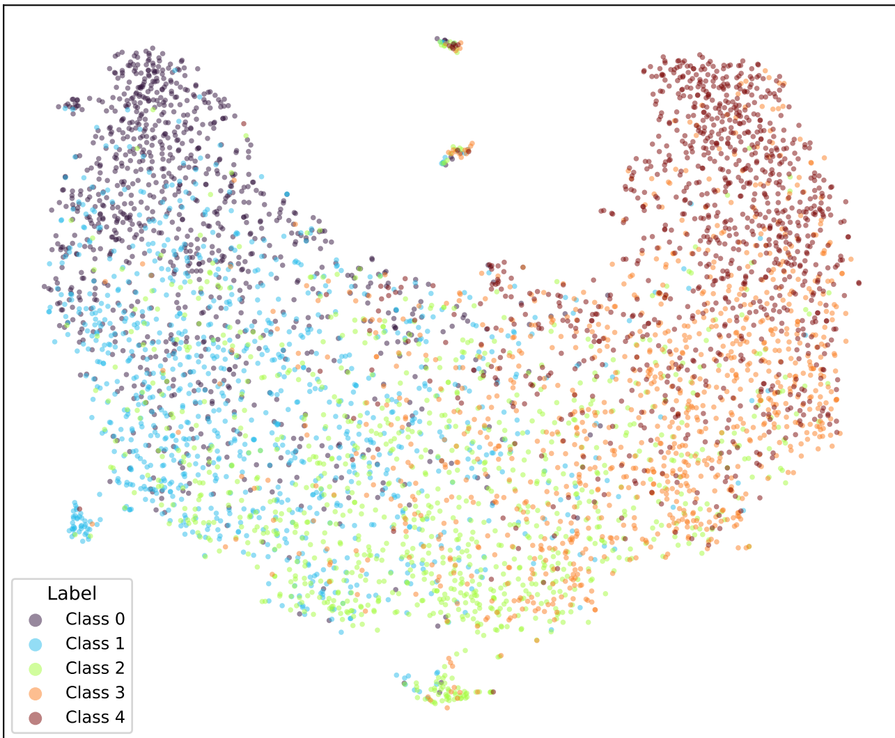
google/bert_uncased_L-2_H-128_A-2-yelp-CE-TRIPa1-1 (val)
