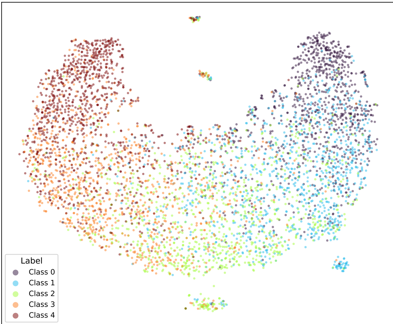
google/bert_uncased_L-2_H-128_A-2-yelp-CE-TRIPa1-3 (val)
