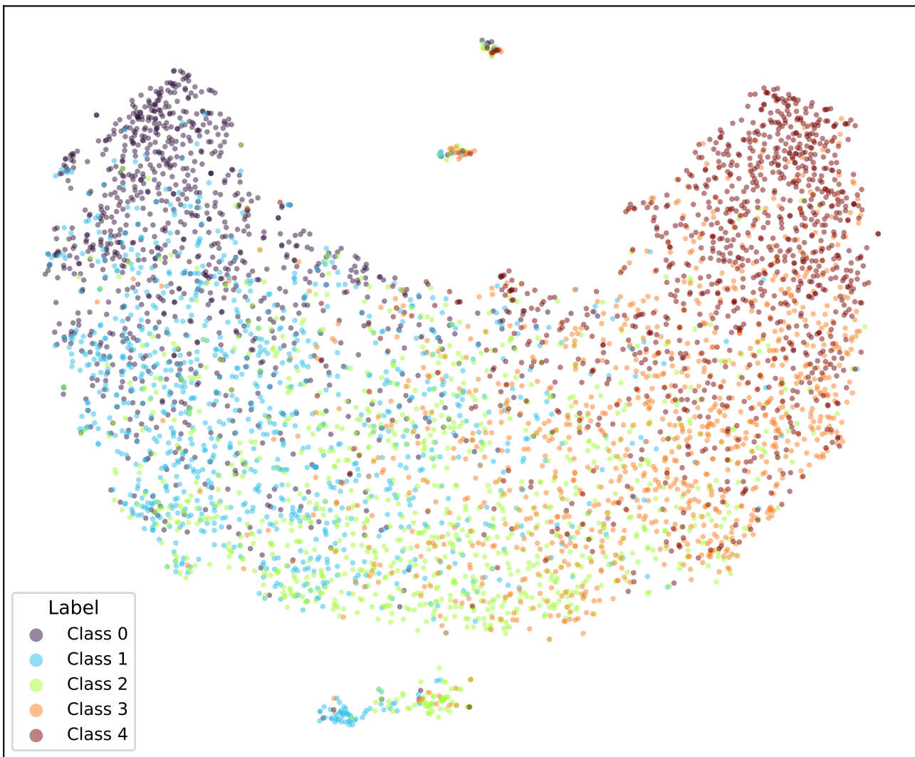
google/bert_uncased_L-2_H-128_A-2-yelp-CE-TRIPa1-4 (val)
