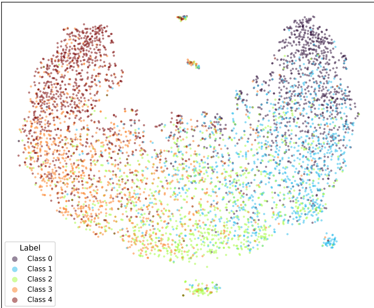
google/bert_uncased_L-2_H-128_A-2-yelp-CE-TRIPa2-3 (val)
