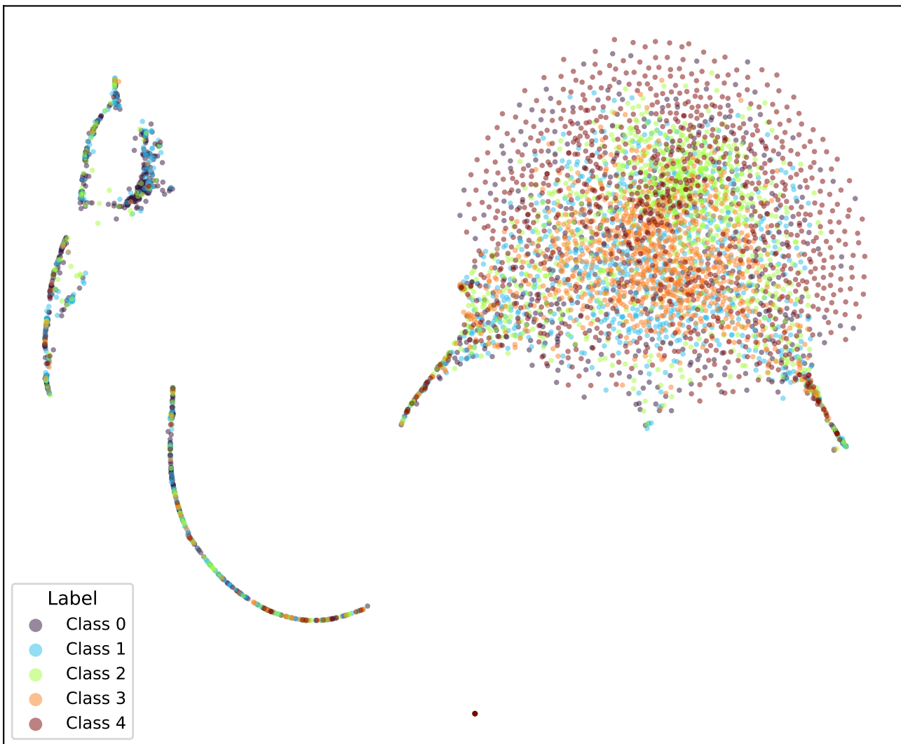
google/bert_uncased_L-2_H-128_A-2-yelp-CORAL-TRIPa1-5 (val)
