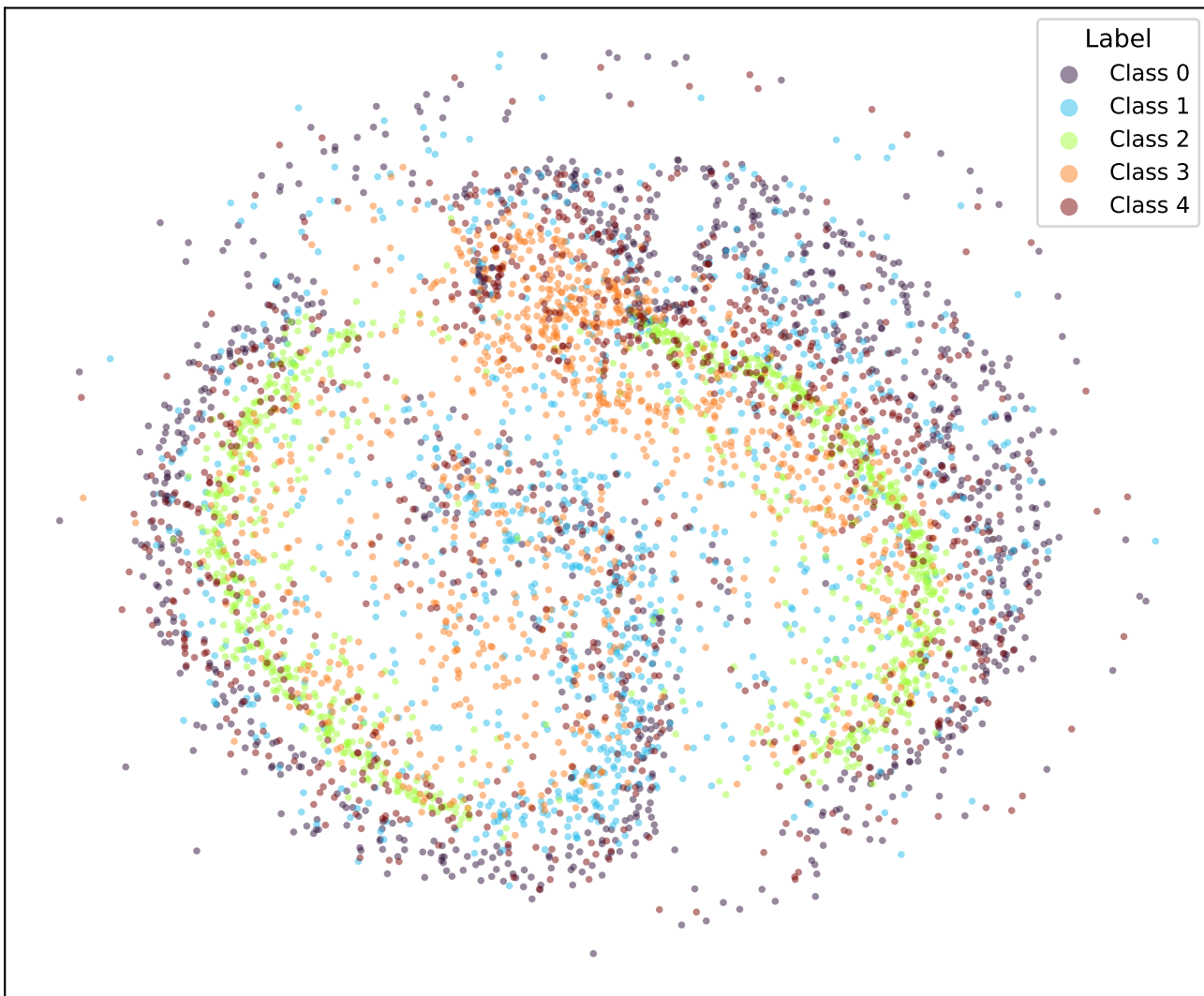
google/bert_uncased_L-2_H-128_A-2-yelp-CORAL-TRIPa2-4 (val)
