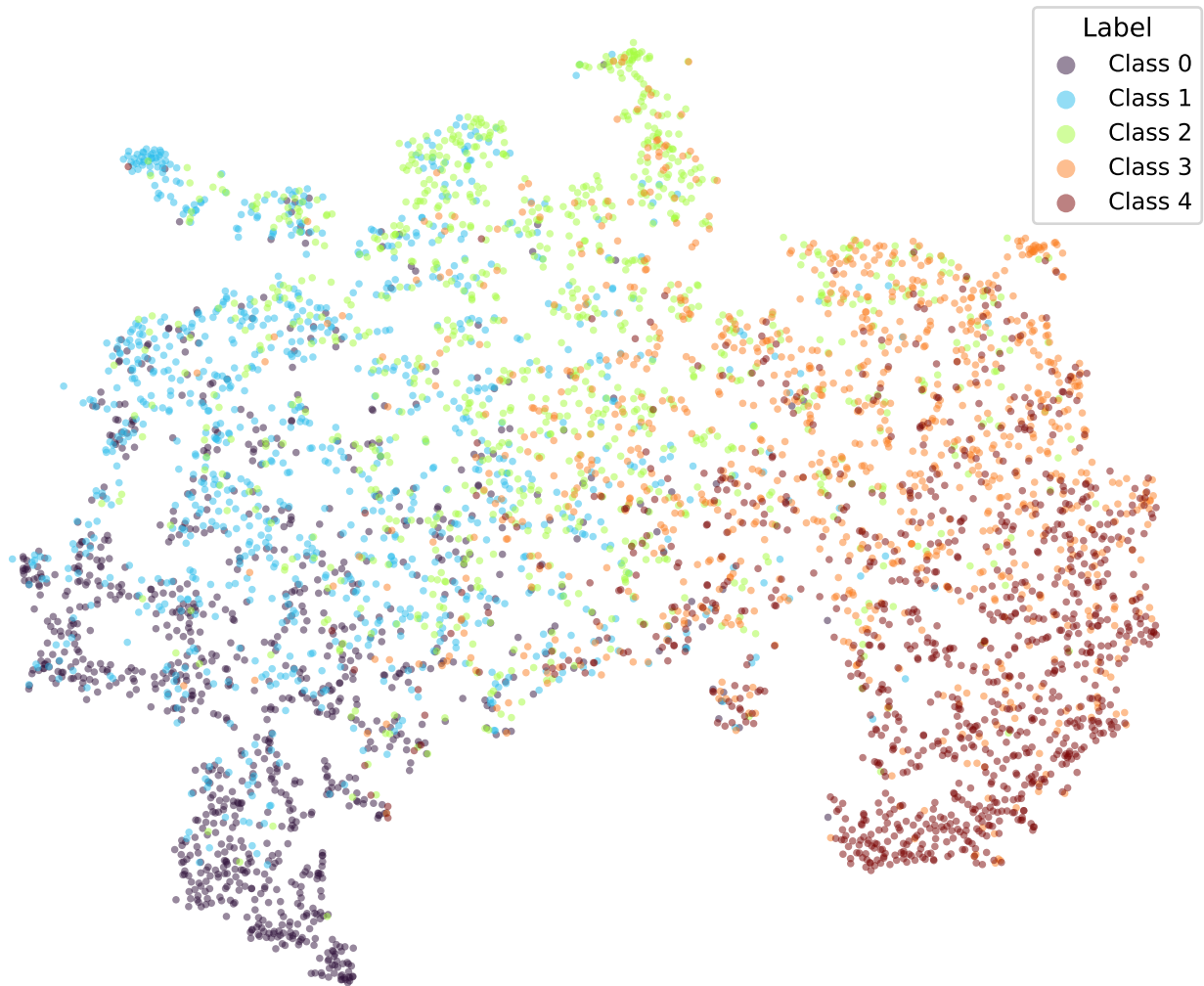
google/bert_uncased_L-2_H-128_A-2-yelp-CORN-2 (val)
