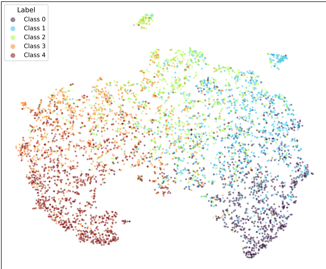
google/bert_uncased_L-2_H-128_A-2-yelp-CORN-3 (val)
