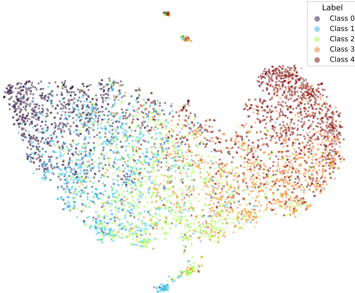
google/bert_uncased_L-2_H-128_A-2-yelp-CORN-3 (val)
