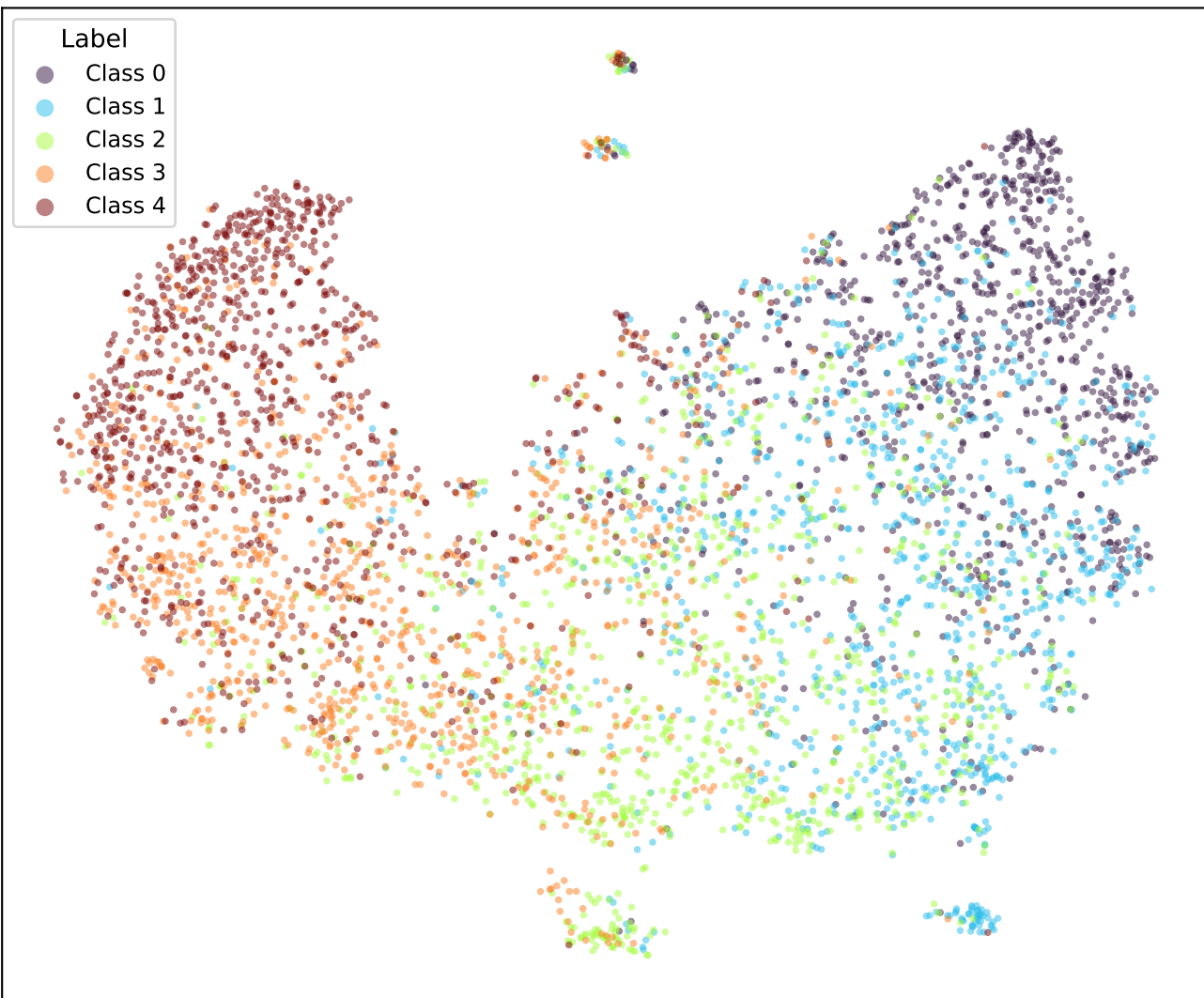
google/bert_uncased_L-2_H-128_A-2-yelp-CORN-4 (val)
