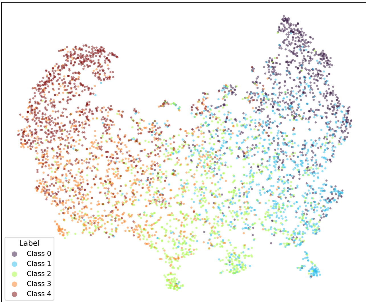
google/bert_uncased_L-2_H-128_A-2-yelp-CORN-4 (val)
