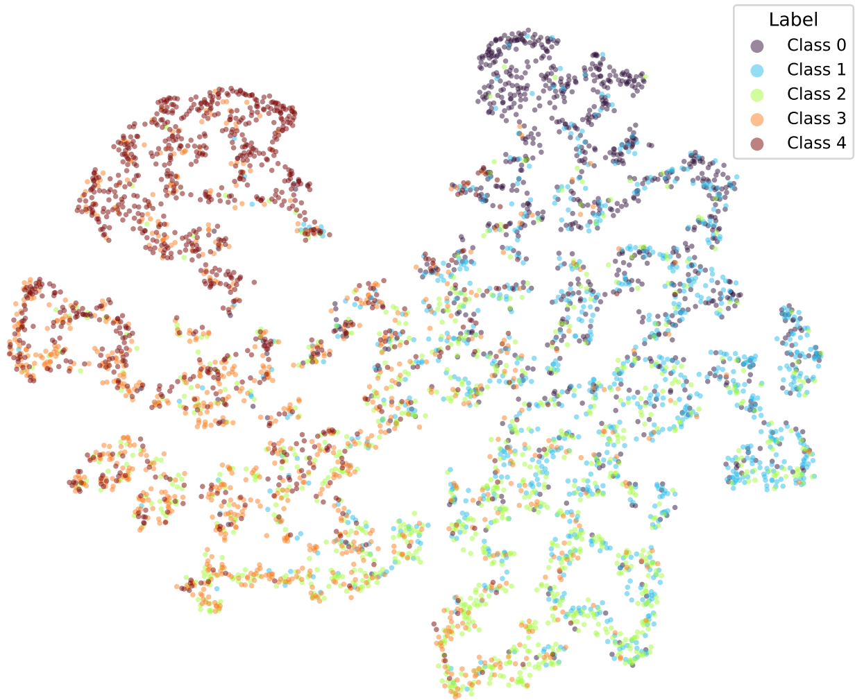
google/bert_uncased_L-2_H-128_A-2-yelp-CORN-4 (val)
