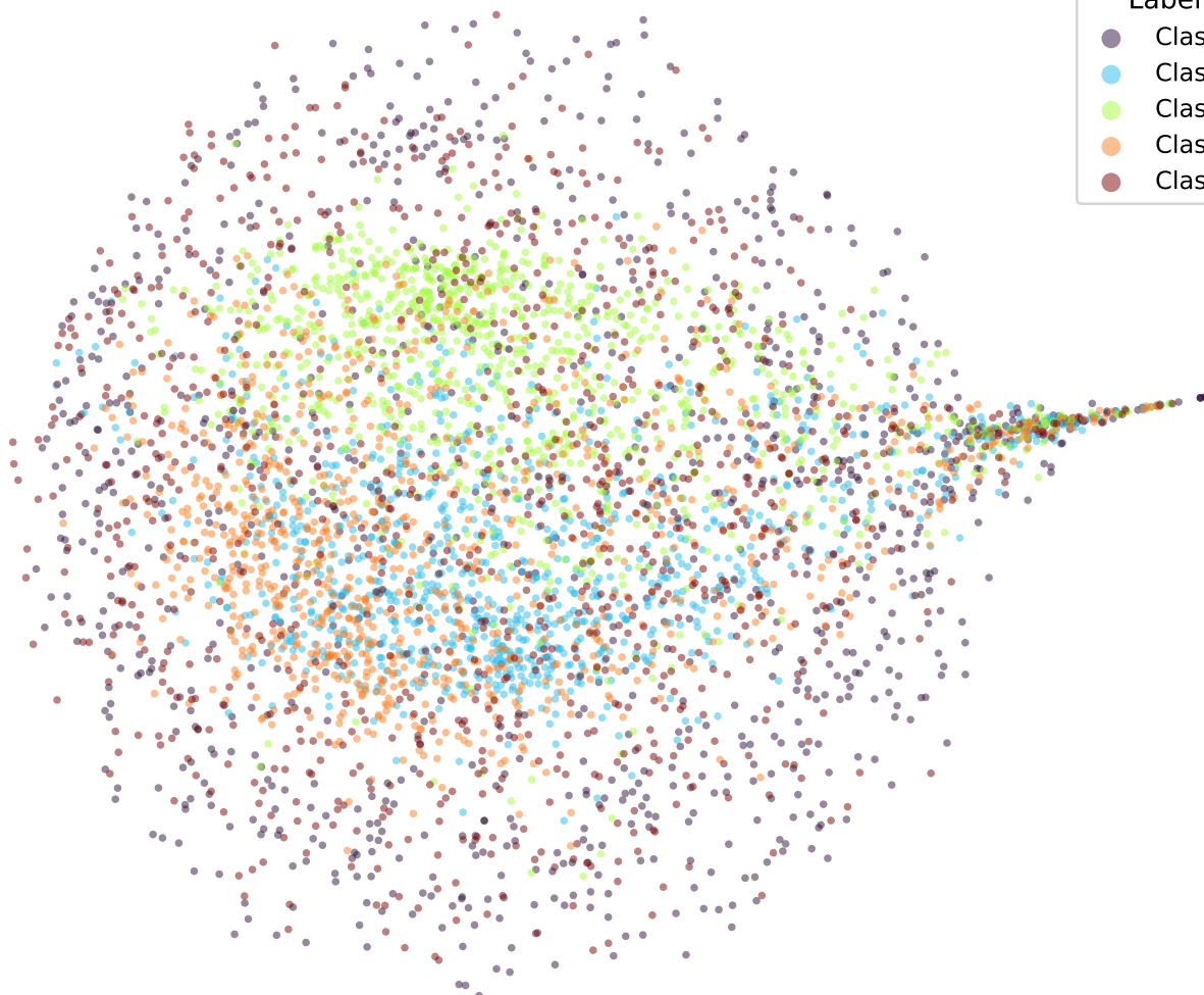
google/bert_uncased_L-2_H-128_A-2-yelp-CORN-5 (val)
