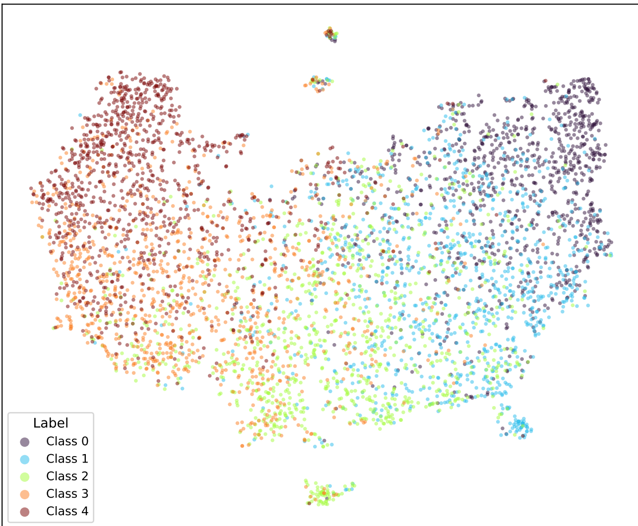
google/bert_uncased_L-2_H-128_A-2-yelp-CORN-5 (val)
