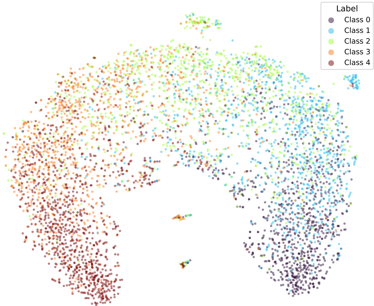
google/bert_uncased_L-2_H-128_A-2-yelp-EMD-TRIPa1-5 (val)
