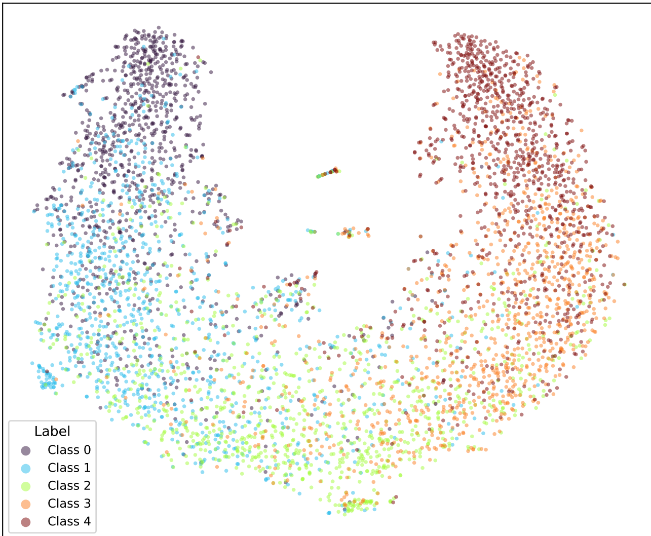
google/bert_uncased_L-2_H-128_A-2-yelp-EMD-TRIPa2-1 (val)
