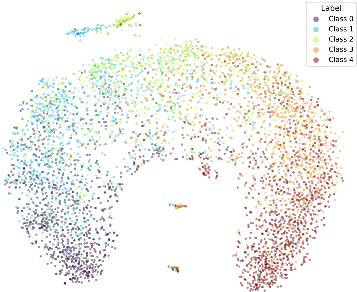
google/bert_uncased_L-2_H-128_A-2-yelp-EMD-TRIPa2-2 (val)
