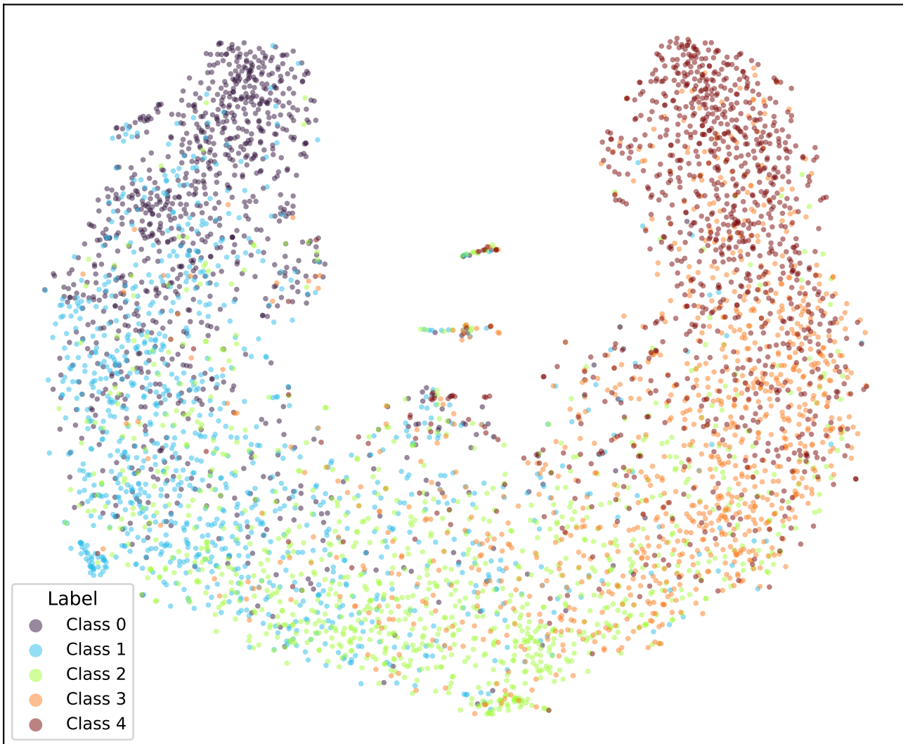
google/bert_uncased_L-2_H-128_A-2-yelp-EMD-TRIPa2-3 (val)
