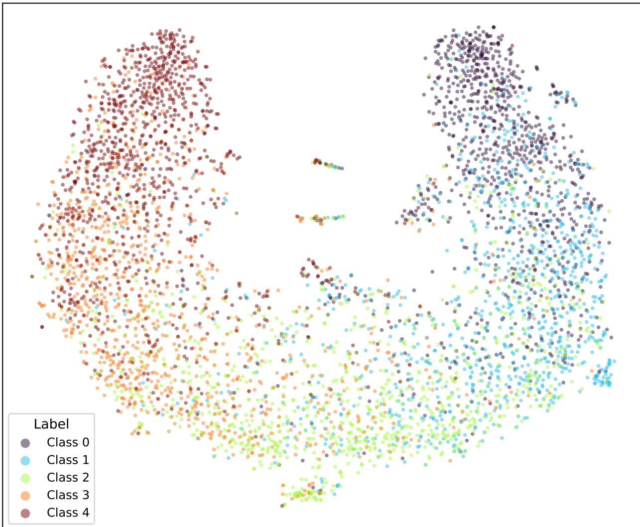
google/bert_uncased_L-2_H-128_A-2-yelp-EMD-TRIPa2-4 (val)
