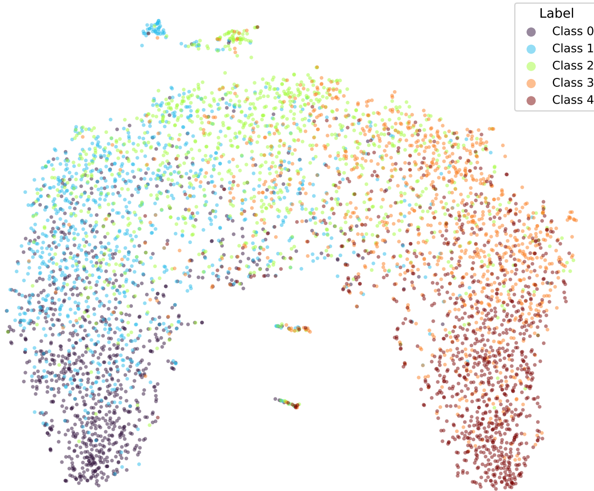
google/bert_uncased_L-2_H-128_A-2-yelp-OLL1-TRIPa1-1 (val)
