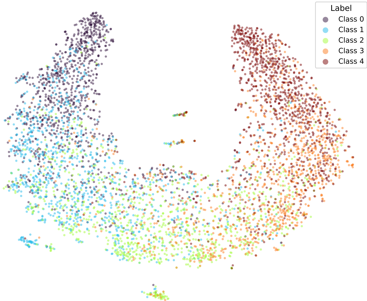
google/bert_uncased_L-2_H-128_A-2-yelp-OLL15-TRIPa1-5 (val)
