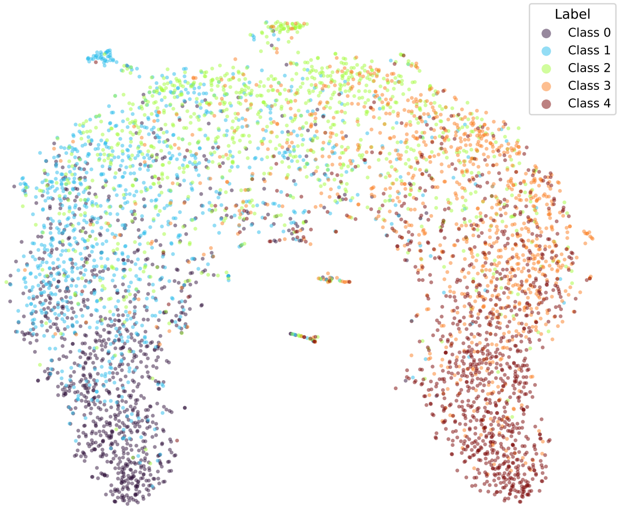
google/bert_uncased_L-2_H-128_A-2-yelp-OLL15-TRIPa2-1 (val)
