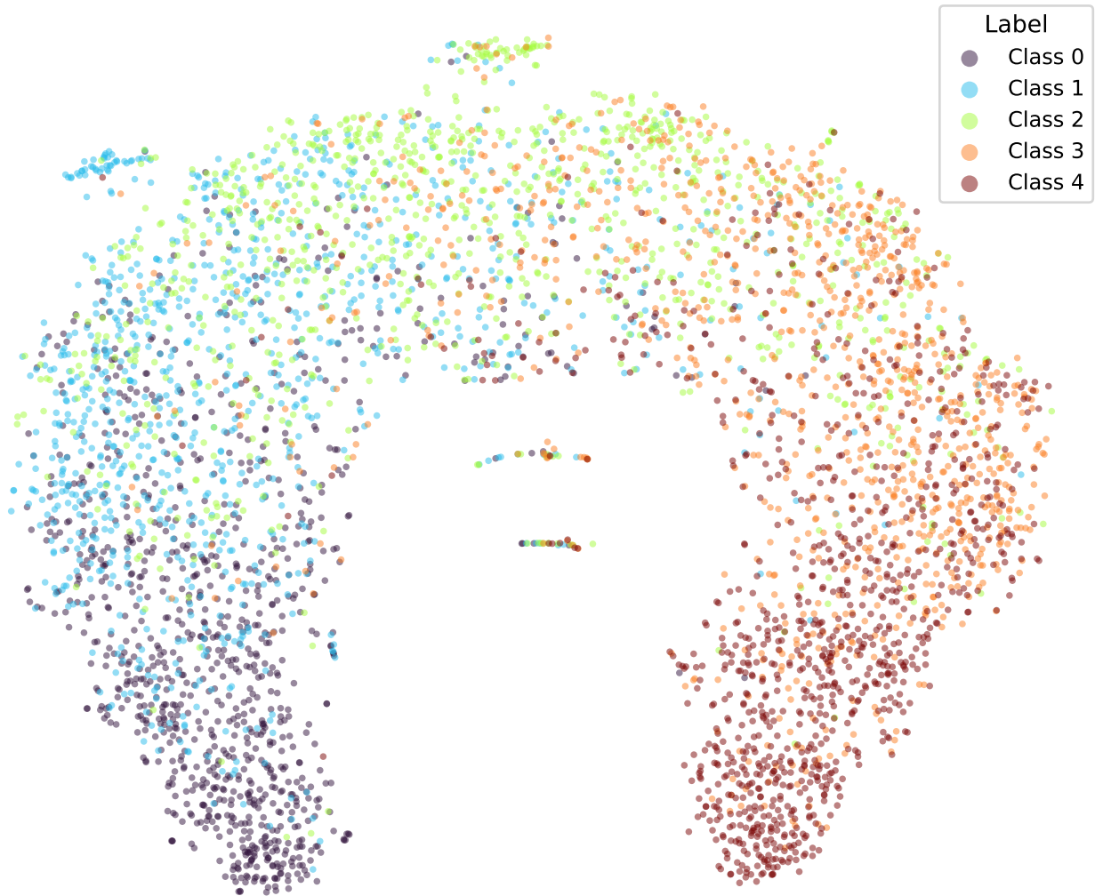
google/bert_uncased_L-2_H-128_A-2-yelp-OLL2-TRIPa1-1 (val)
