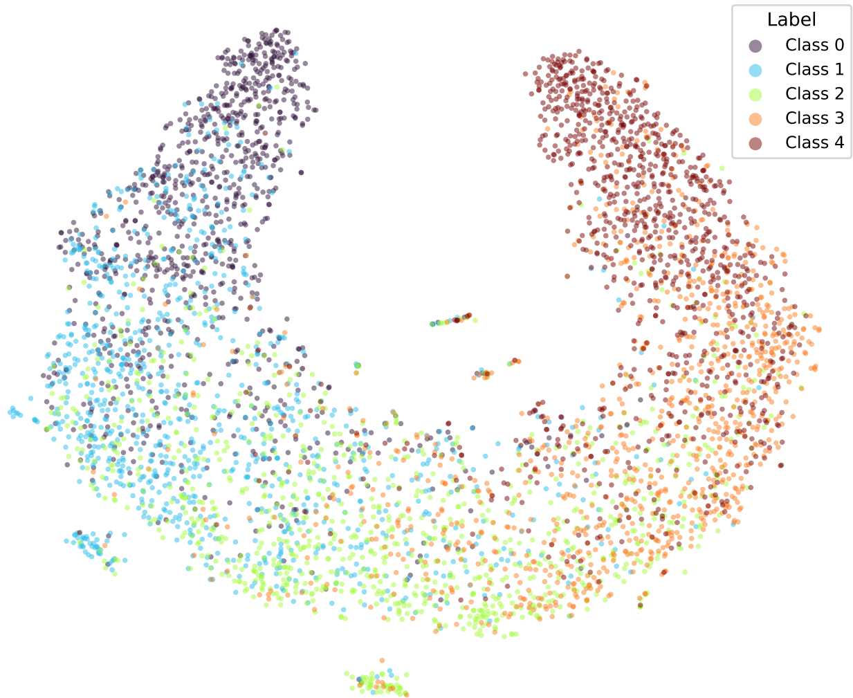
google/bert_uncased_L-2_H-128_A-2-yelp-OLL2-TRIPa1-3 (val)
