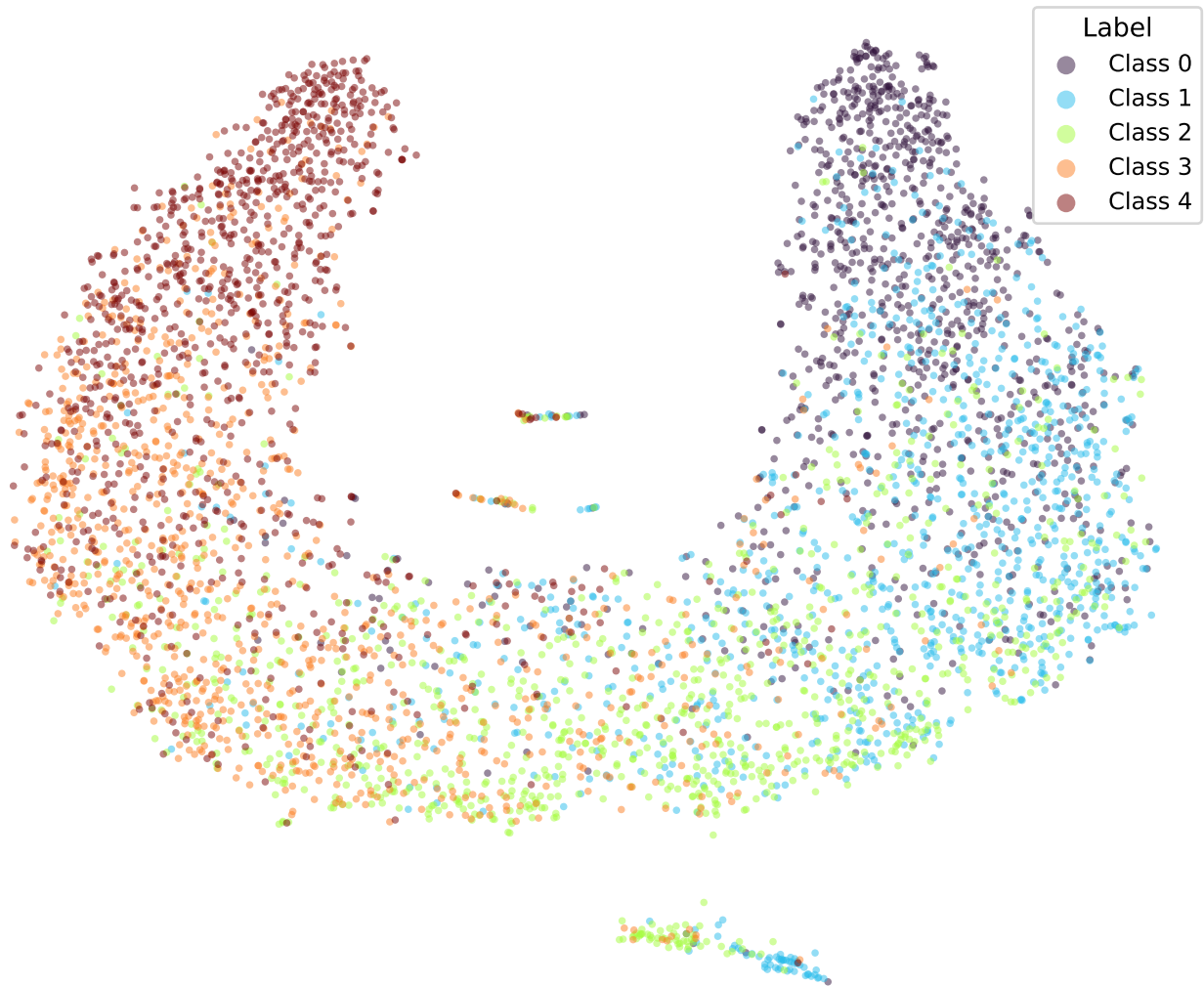
google/bert_uncased_L-2_H-128_A-2-yelp-OLL2-TRIPa1-4 (val)
