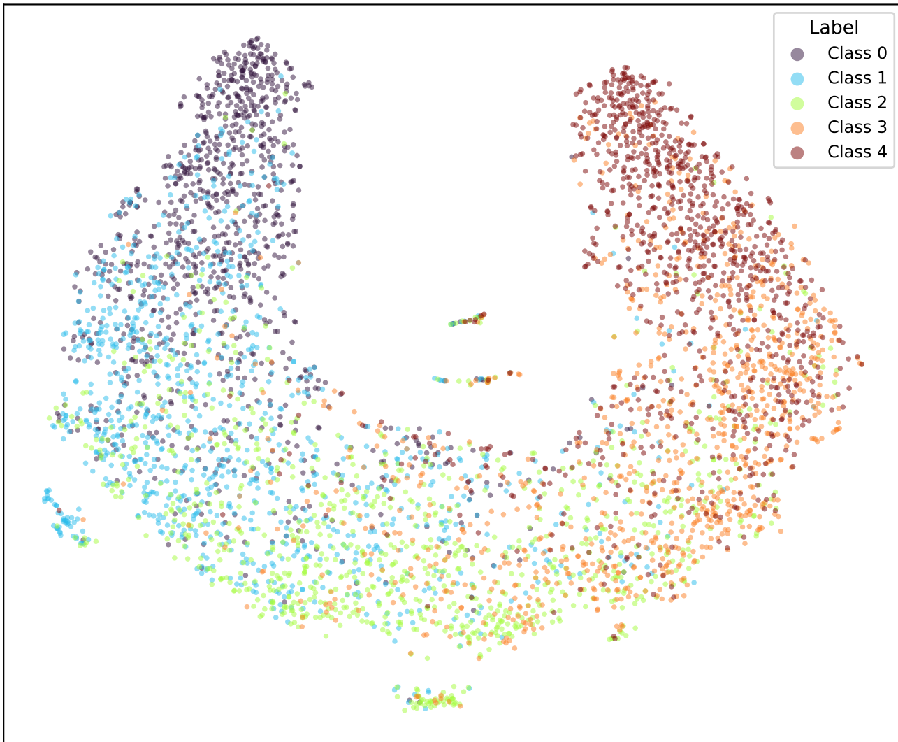
google/bert_uncased_L-2_H-128_A-2-yelp-OLL2-TRIPa1-5 (val)
