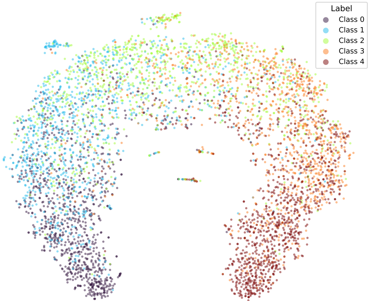
google/bert_uncased_L-2_H-128_A-2-yelp-OLL2-TRIPa2-1 (val)
