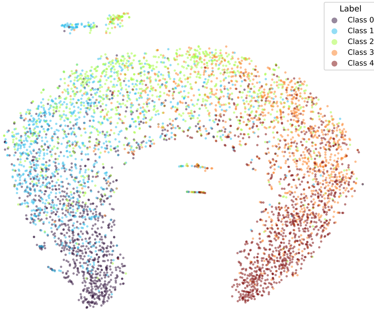
google/bert_uncased_L-2_H-128_A-2-yelp-OLL2-TRIPa2-2 (val)
