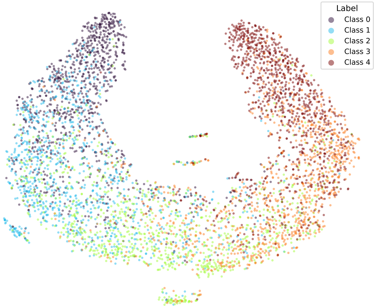
google/bert_uncased_L-2_H-128_A-2-yelp-OLL2-TRIPa2-3 (val)
