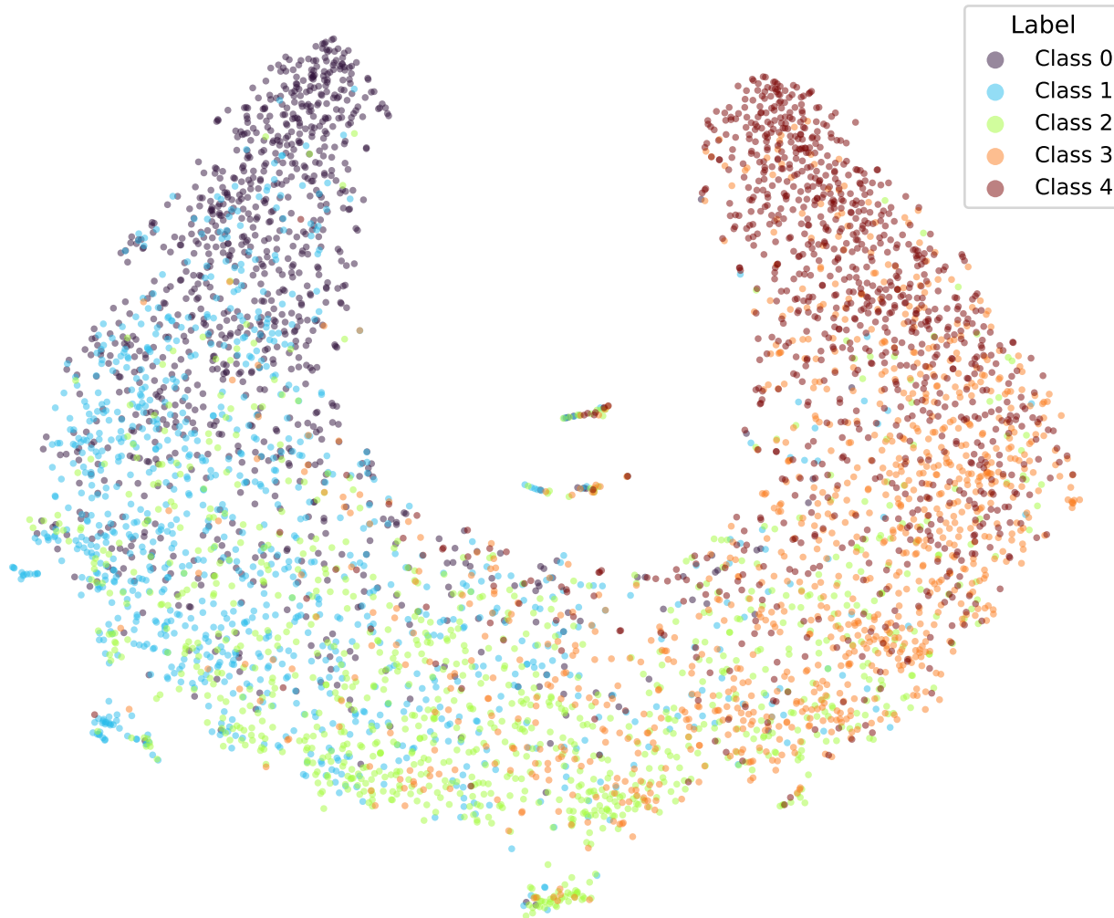
google/bert_uncased_L-2_H-128_A-2-yelp-OLL2-TRIPa2-5 (val)
