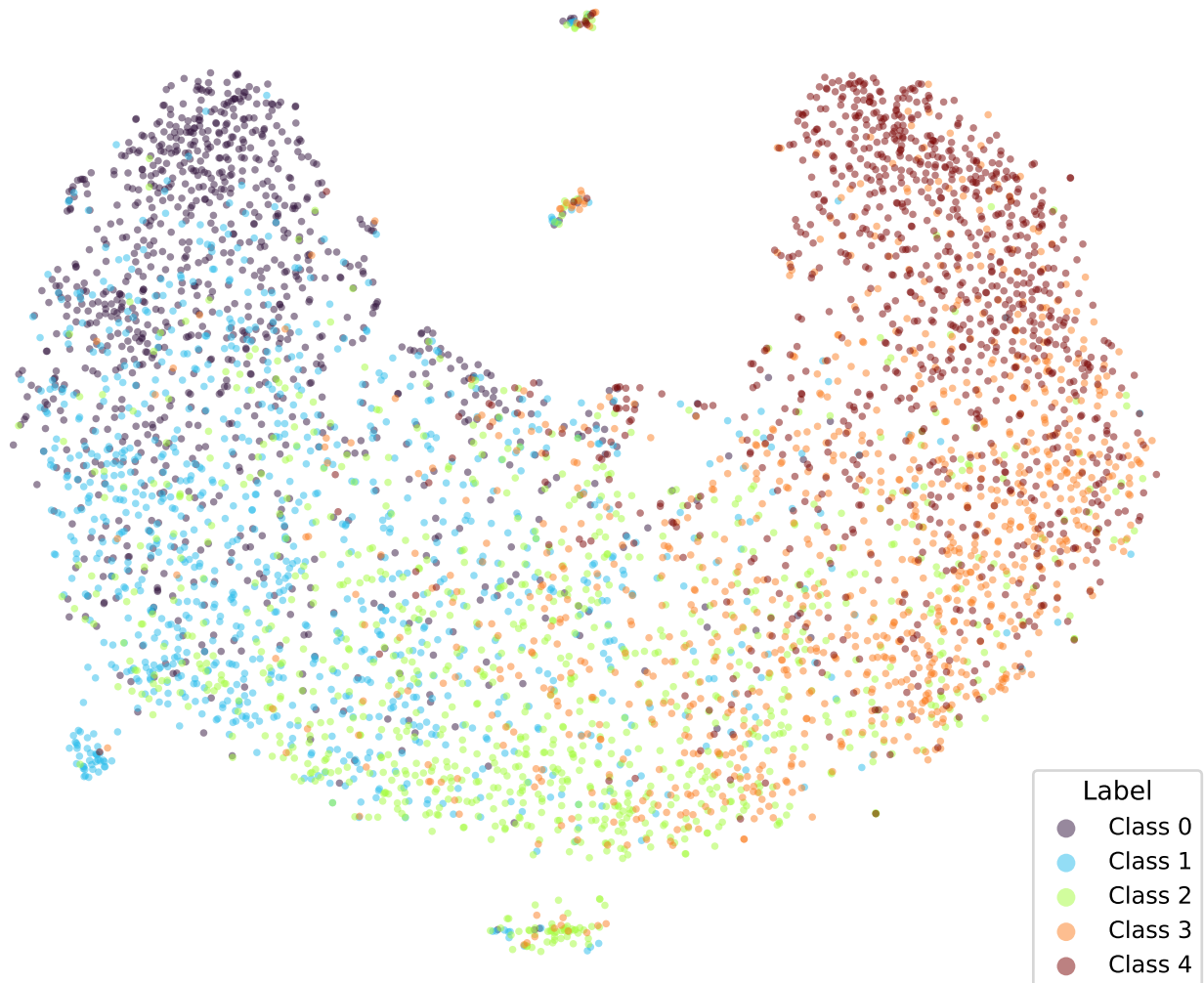
google/bert_uncased_L-2_H-128_A-2-yelp-SOFT2-TRIPa1-3 (val)
