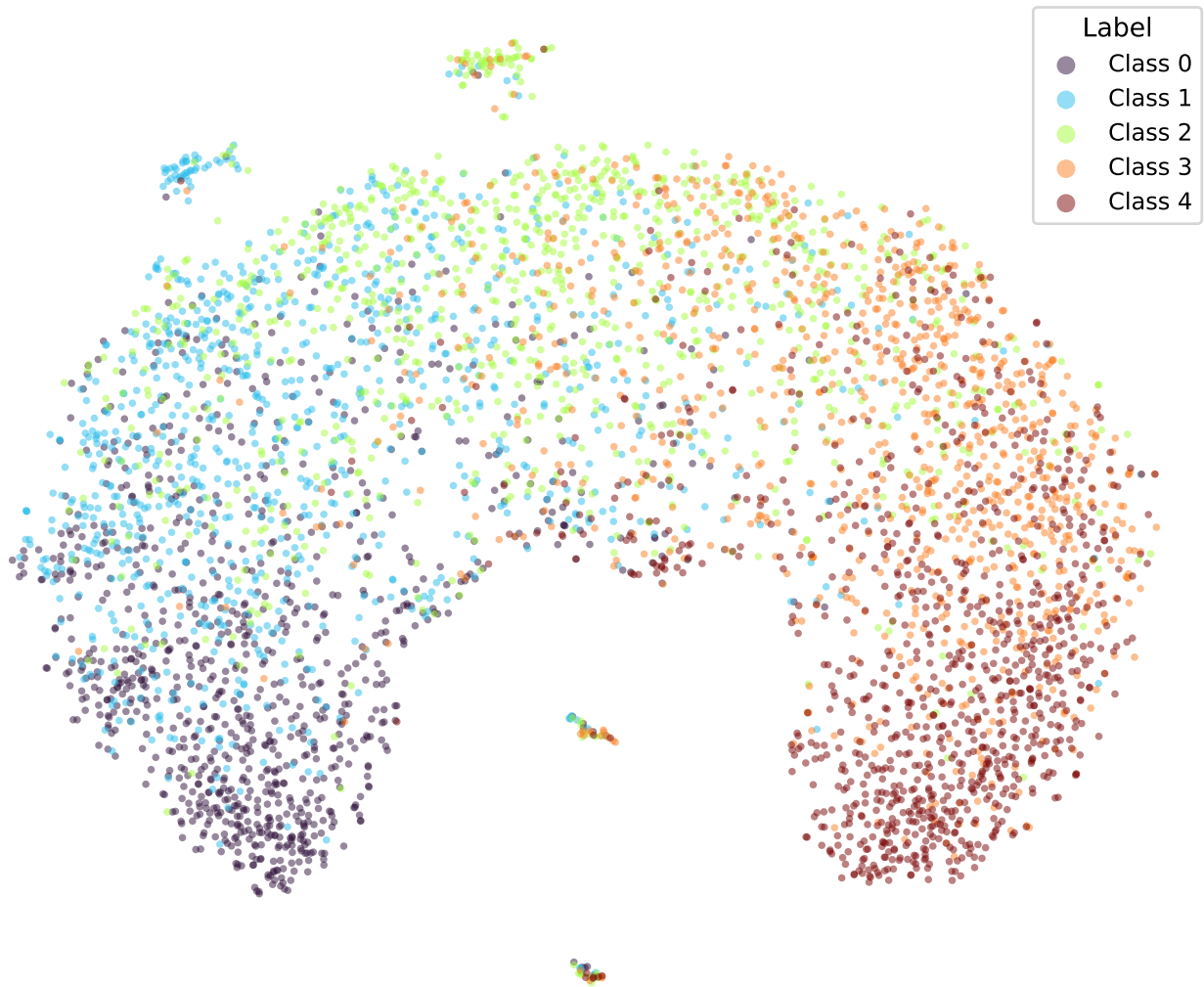
google/bert_uncased_L-2_H-128_A-2-yelp-SOFT2-TRIPa2-2 (val)
