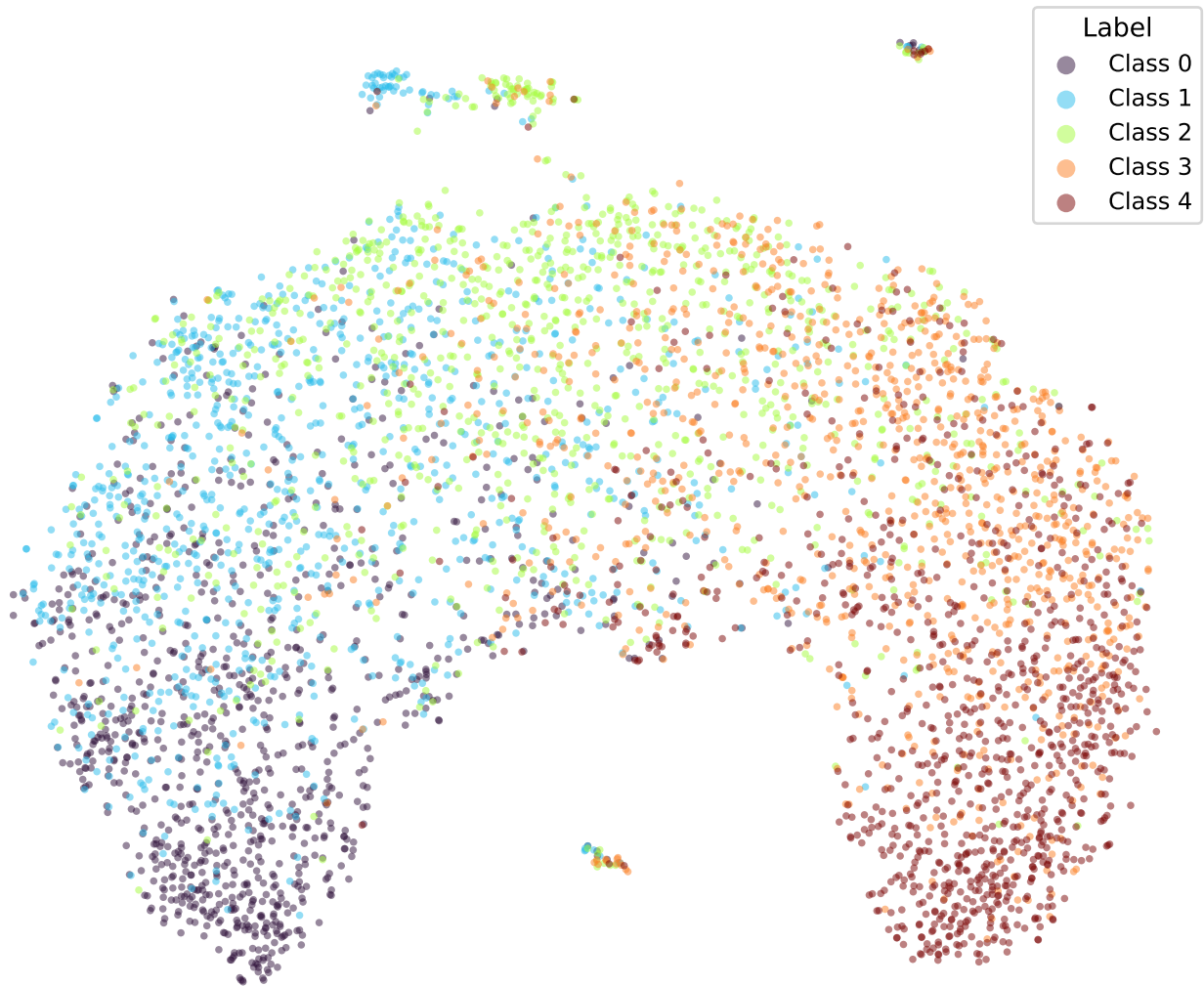
google/bert_uncased_L-2_H-128_A-2-yelp-SOFT3-TRIPa1-2 (val)
