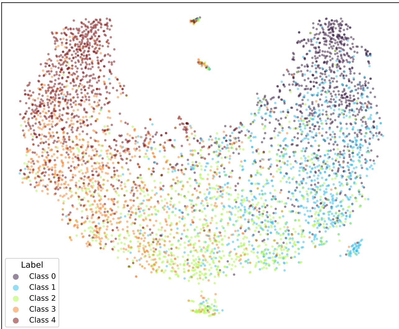
google/bert_uncased_L-2_H-128_A-2-yelp-SOFT3-TRIPa2-1 (val)
