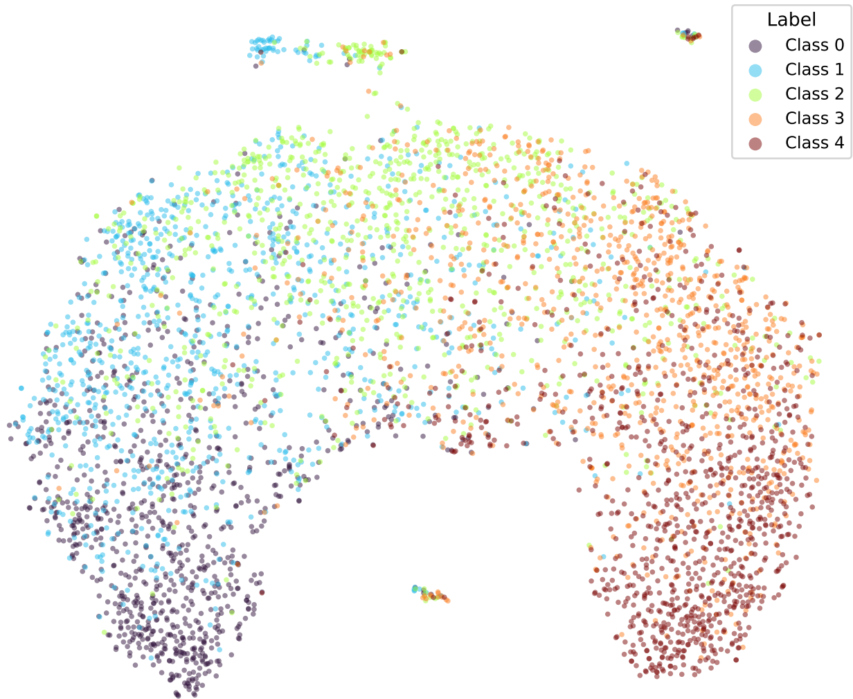
google/bert_uncased_L-2_H-128_A-2-yelp-SOFT3-TRIPa2-2 (val)
