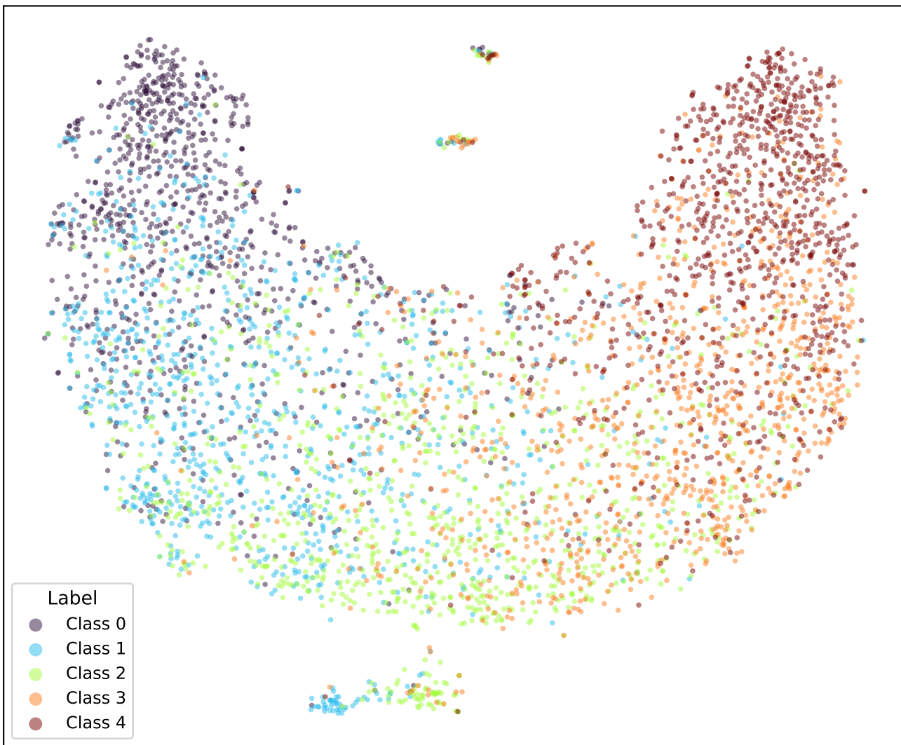
google/bert_uncased_L-2_H-128_A-2-yelp-SOFT3-TRIPa2-4 (val)
