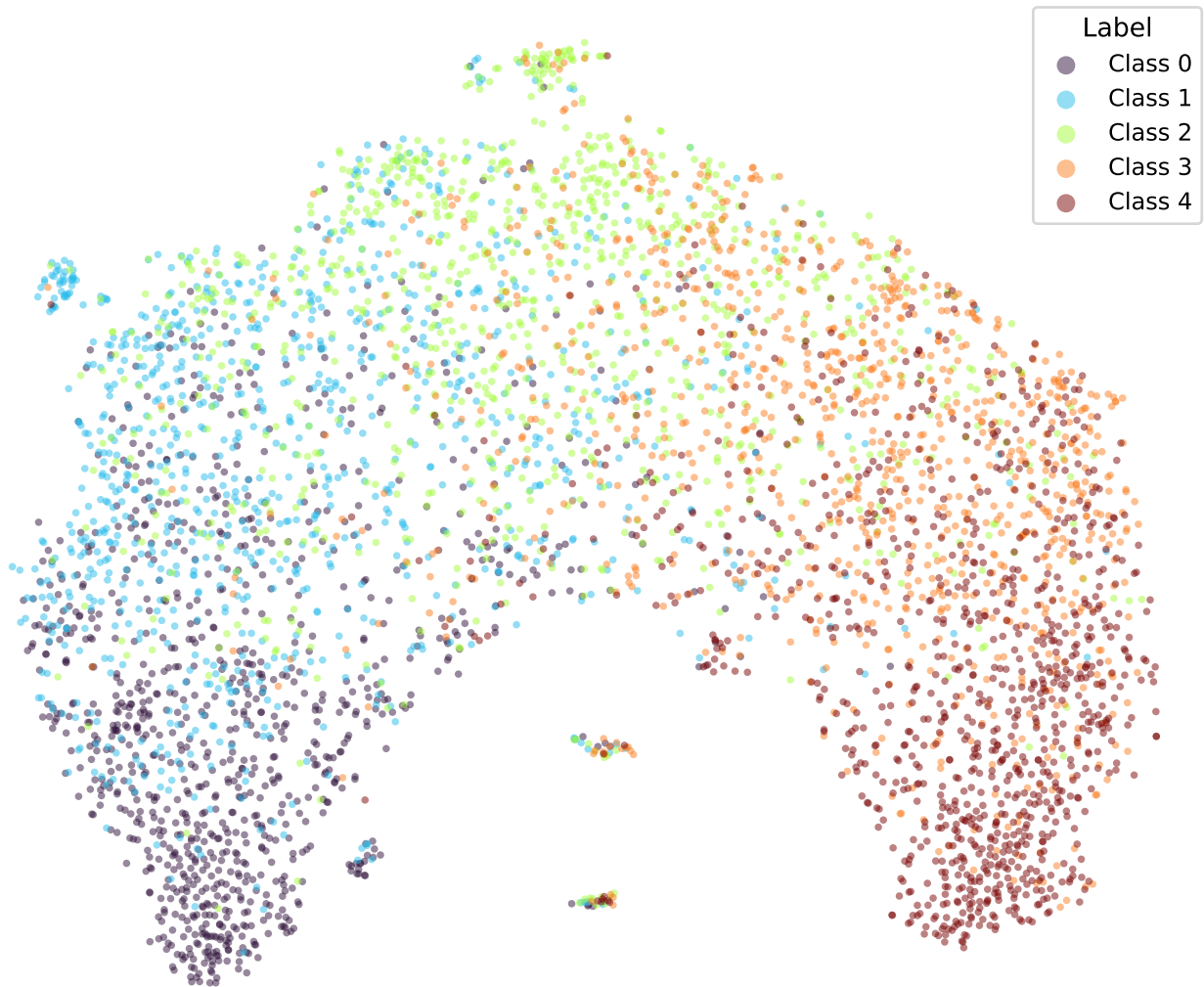
google/bert_uncased_L-2_H-128_A-2-yelp-SOFT4-TRIPa2-1 (val)
