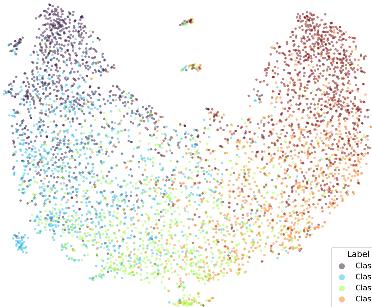
google/bert_uncased_L-2_H-128_A-2-yelp-SOFT4-TRIPa2-4 (val)
