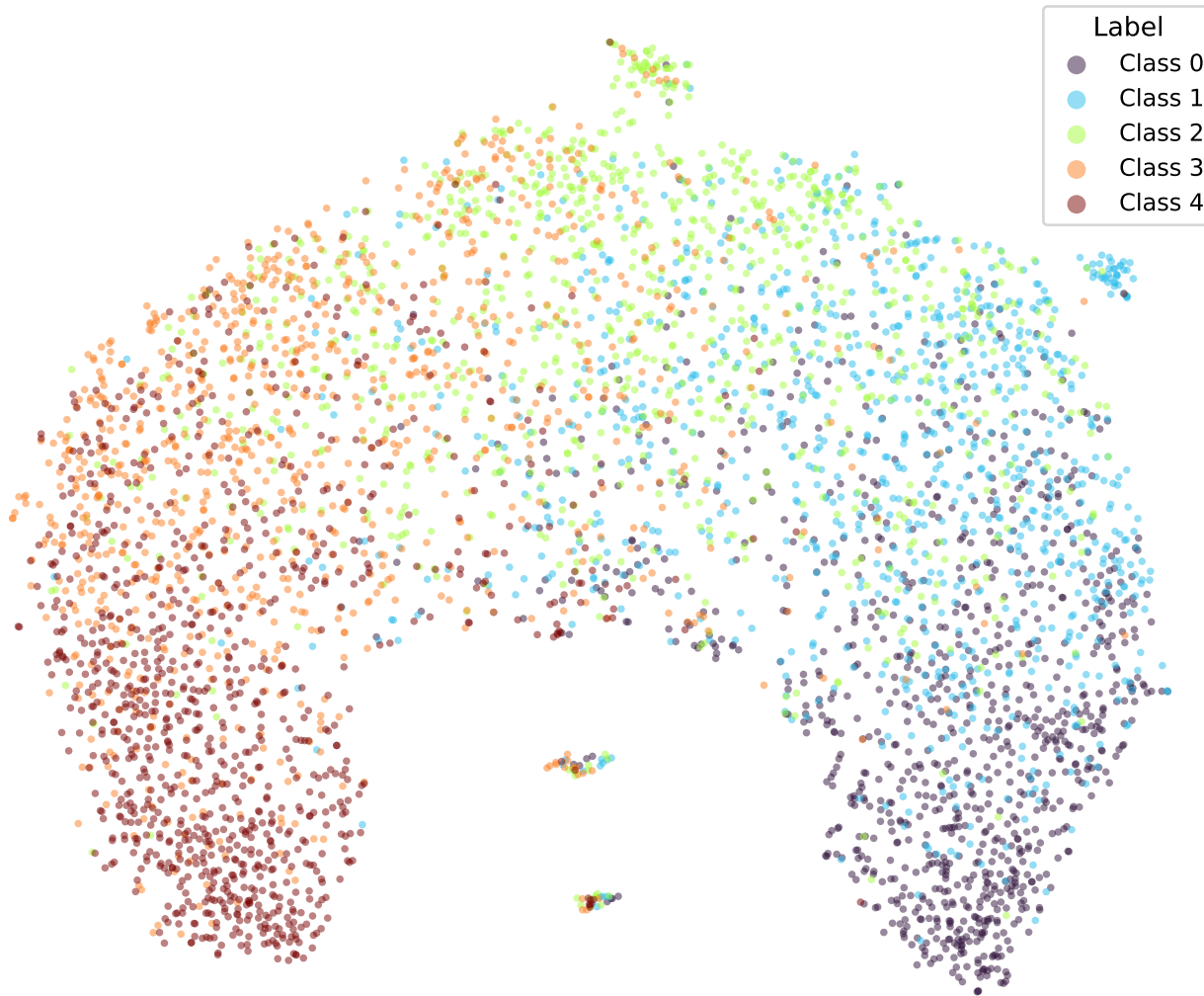
google/bert_uncased_L-2_H-128_A-2-yelp-SOFT4-TRIPa2-5 (val)
