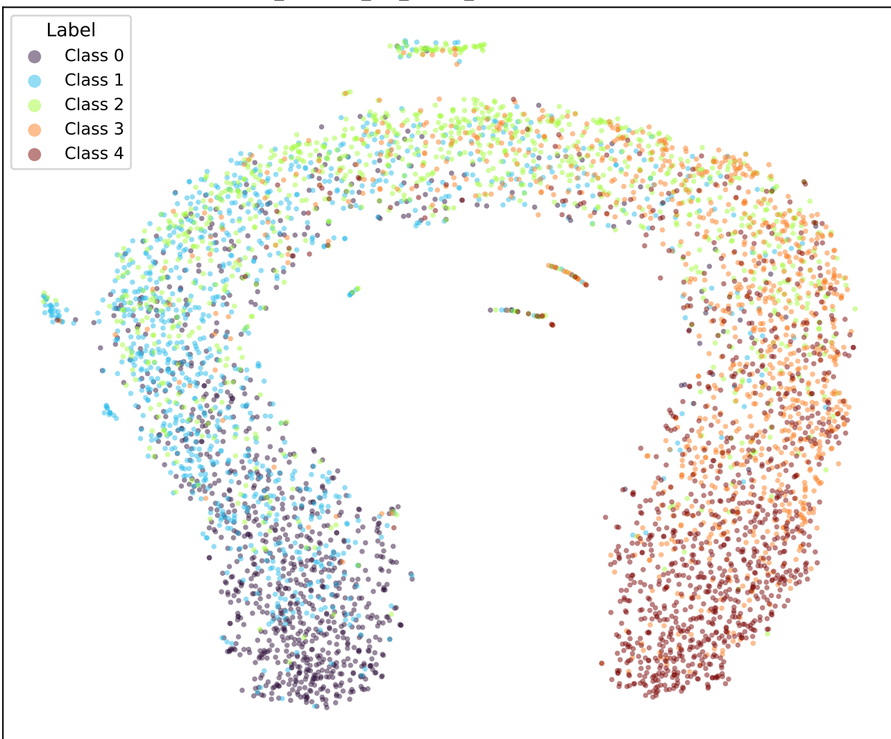
google/bert_uncased_L-2_H-128_A-2-yelp-WKL-TRIPa1-1 (val)
