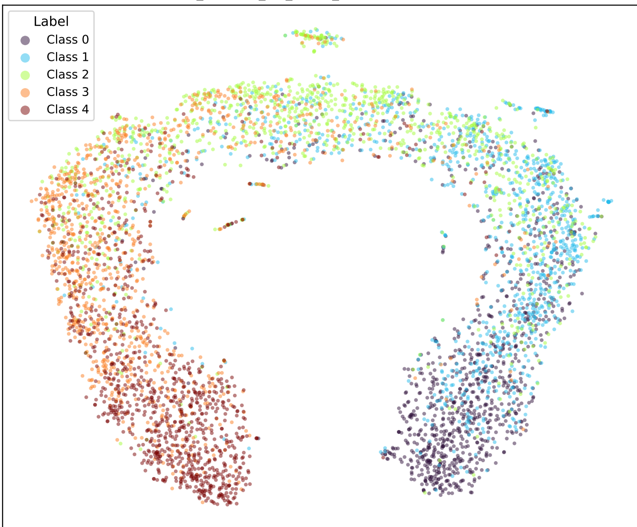
google/bert_uncased_L-2_H-128_A-2-yelp-WKL-TRIPa1-3 (val)
